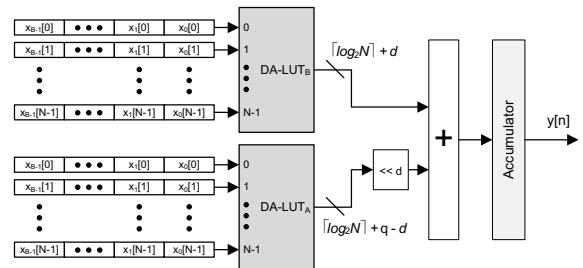
Fig. 4. DA architecture with decomposed lookup table.
