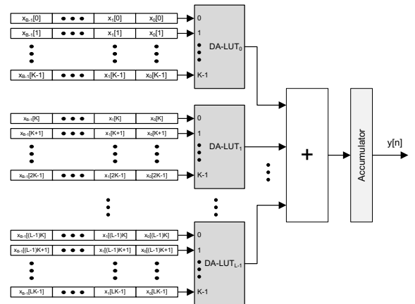
Fig. 3. DA architecture with partitioned lookup table.
