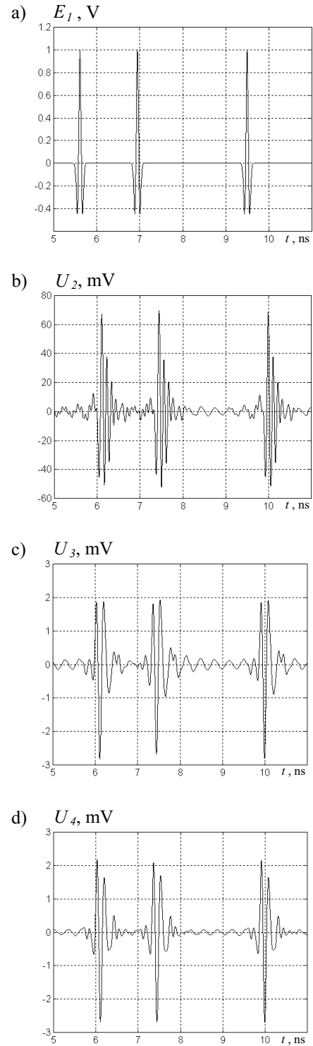
Fig. 6. Pulse propagation in MIMO UWB antenna system.
