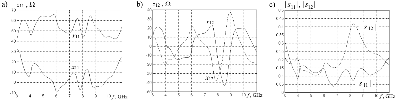
Fig. 2. Elements of impedance a), b) and scattering c) matrices of two-element UWB antenna.
