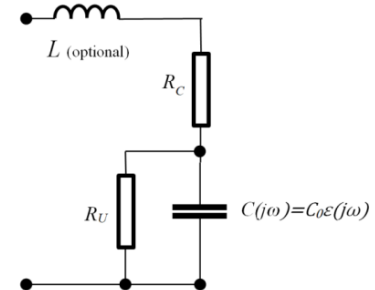
Fig. 2. Equivalent circuit of a supercapacitor
