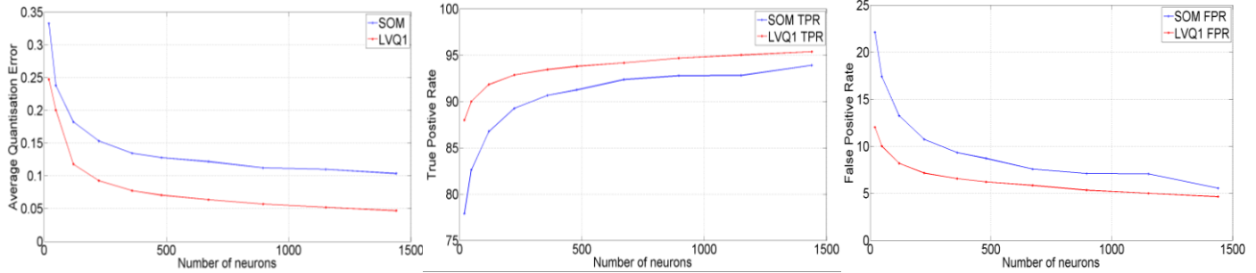
Fig. 4. Average Quantisation Error , TPR, FPR versus the number of neuron
