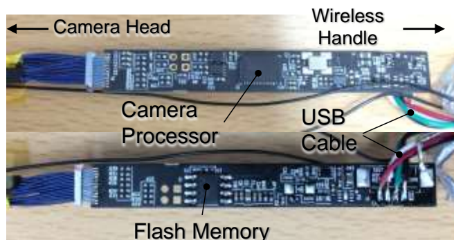
Fig. 5. Top and bottom side of the camera controller for the wireless endoscope.
