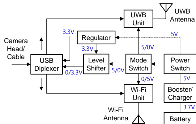
Fig. 6. Configuration of the wireless handle.
