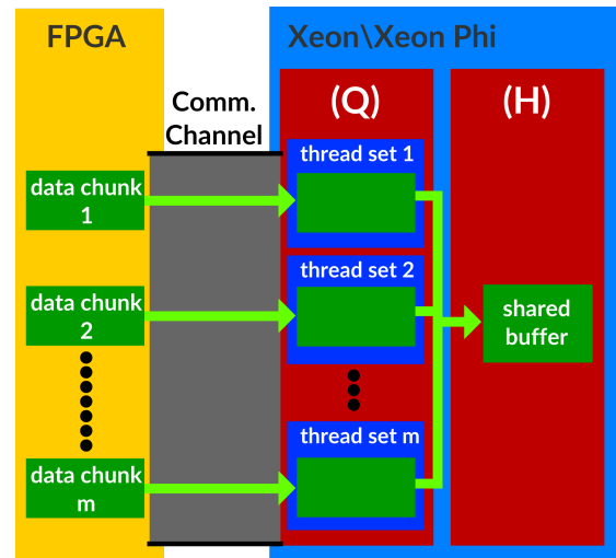
Fig. 12. Overview of system communication and data flow. Variable m should be chosen to fulfill real-time requirements described in figure 10. Scope of this work consists only of Q part.
