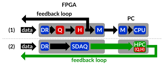
Fig. 5. Legacy system with optimization proposition. Migration of calculation part create additional latency and communication overhead. Along with such change new algorithmic possibilities emerge.
