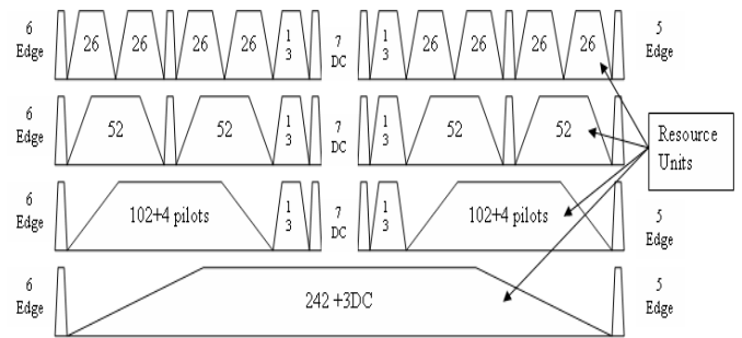
Fig. 1 Structure of the 802.11ax PHY layer in the 20MHz channel
