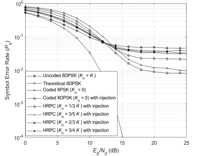
Fig. 8. Symbol error rate curves for injection coding schemes under AWGN, frequency selective fading and impulsive noise channel.
