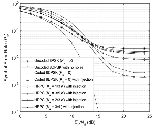
Fig. 9. Symbol error rate curves for injection coding schemes under AWGN and frequency selective fading channel.
