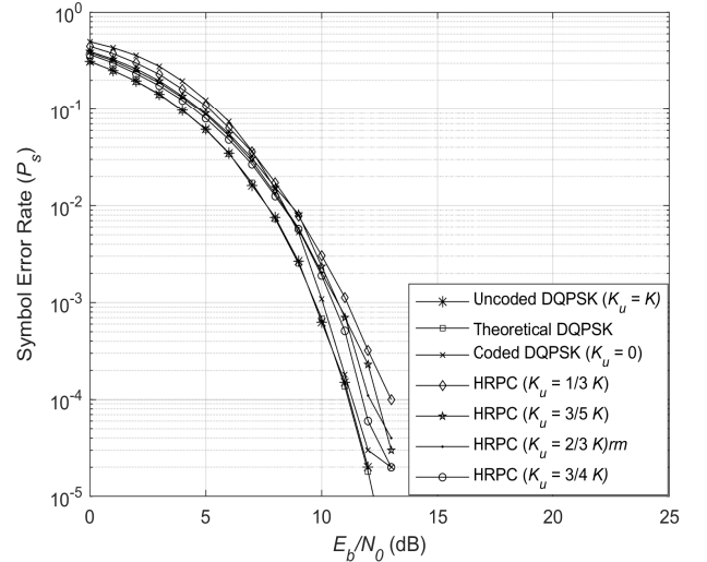
Fig. 3. Symbol error rate curves for DQPSK schemes under AWGN.
