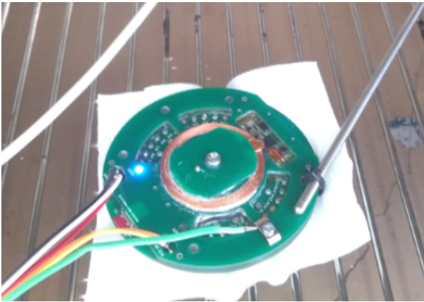
Fig. 10. Test of RTD installed on PCB
