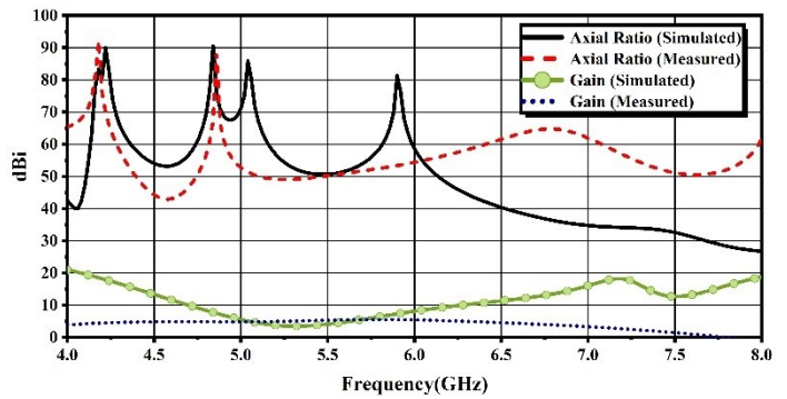
Fig. 21. Simulated and Measured Axial Ratio as well as Peak gain when switch is OFF.
