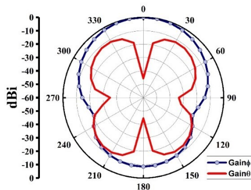
Fig. 9. Simulated Normalized radiation pattern when switch is OFF at H-plane
