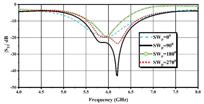
Fig. 7. Simulated |S_{11}| for different values of SW_p when switch is in ON state.
