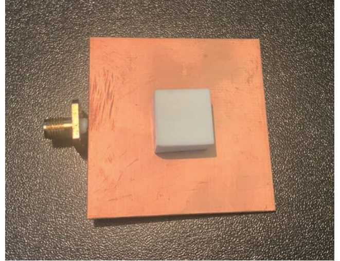
Fig. 14. Fabricated Prototype
