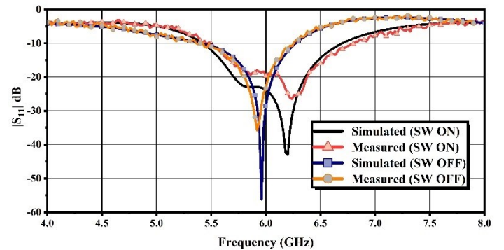
Fig. 15. Simulated and Measured reflection coefficient
