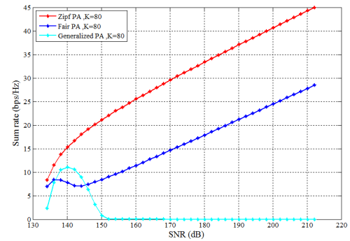
Fig. 6. Sum rate versus SNR pour Zipf PA, Fair PA and Generalized PA
