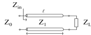
Fig. 2. Wideband adaptation
