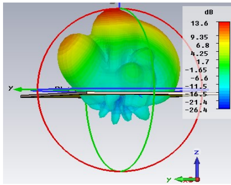
Fig. 14. Gain simulation 3D result of the array antenna four elements
