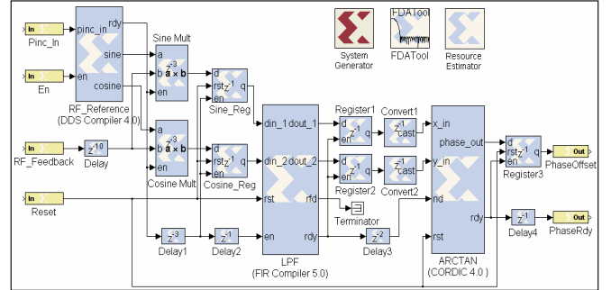
Fig. 10. Phase measurement using CORDIC algorithm.
