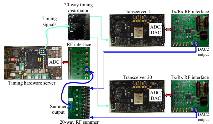
Fig. 22. CORDIC based synchronisation TIGER-3 radar system.
