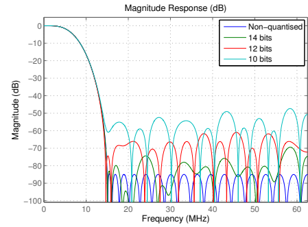
(a) 36-tap FIR lowpass filter
