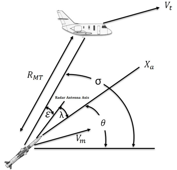
Fig. 4. Missile flight and homing head angles
